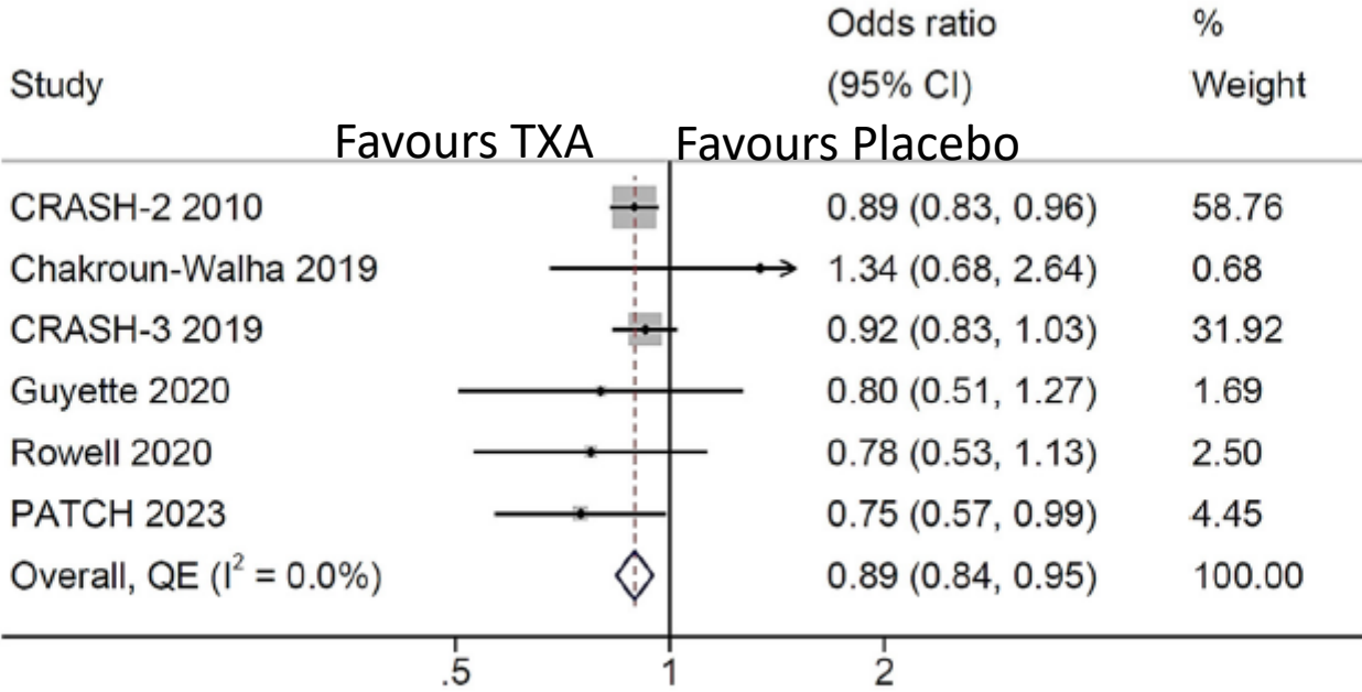
Figure 2. Forest plot depicting estimated effects of each trial and the meta-analytic effect. Odds ratios indicate the odds of mortality with tranexamic acid compared to placebo at one month. CI , confidence interval.
